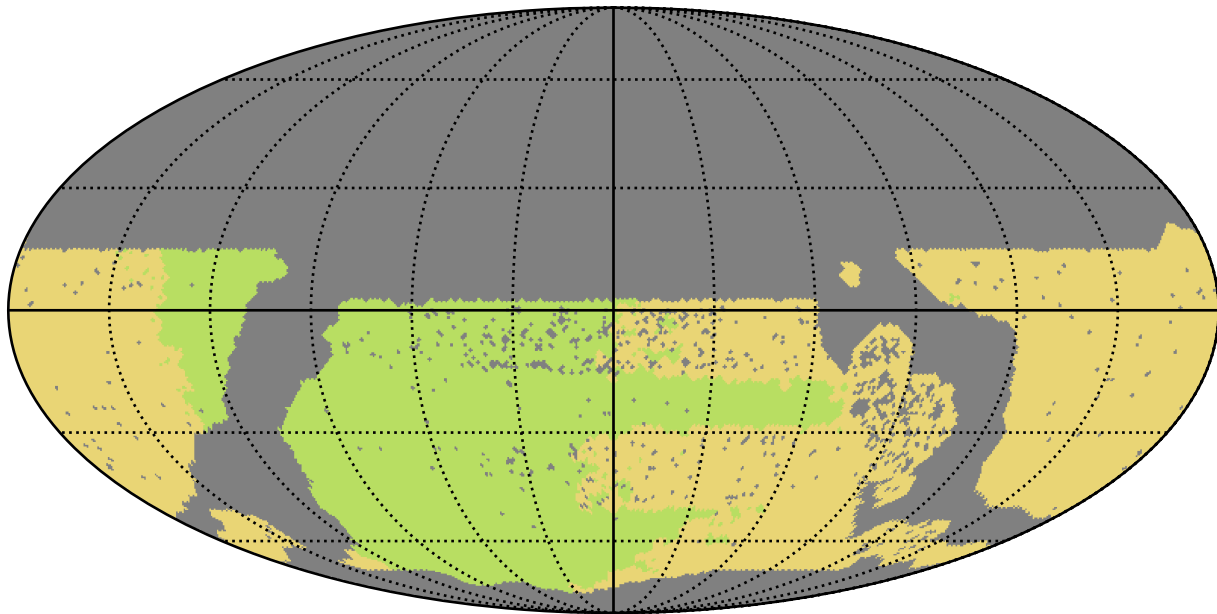
baseline_v3.2_10yrs WFD all bands: NSeasons
