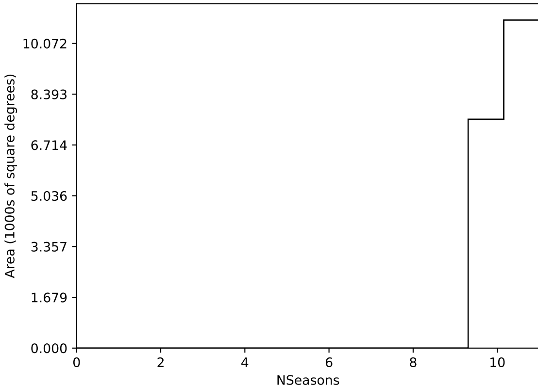
baseline_v3.2_10yrs WFD all bands: NSeasons
