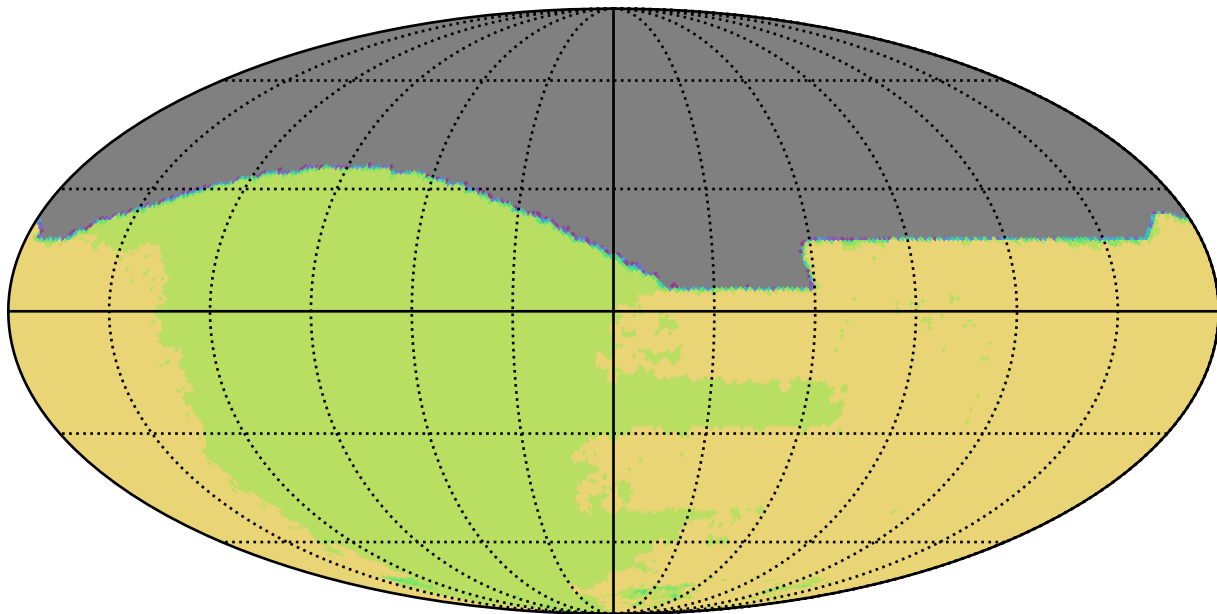
baseline_v3.2_10yrs All sky all bands: NSeasons
