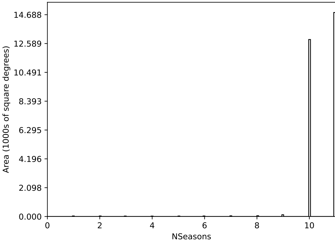
baseline_v3.2_10yrs All sky all bands: NSeasons
