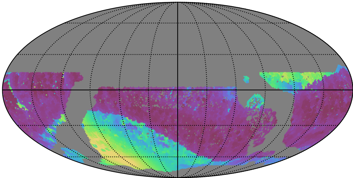
baseline_v3.2_10yrs WFD z band: Min solarElong
