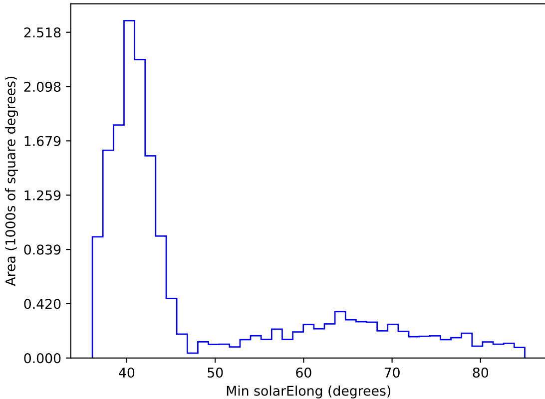
baseline_v3.2_10yrs WFD z band: Min solarElong
