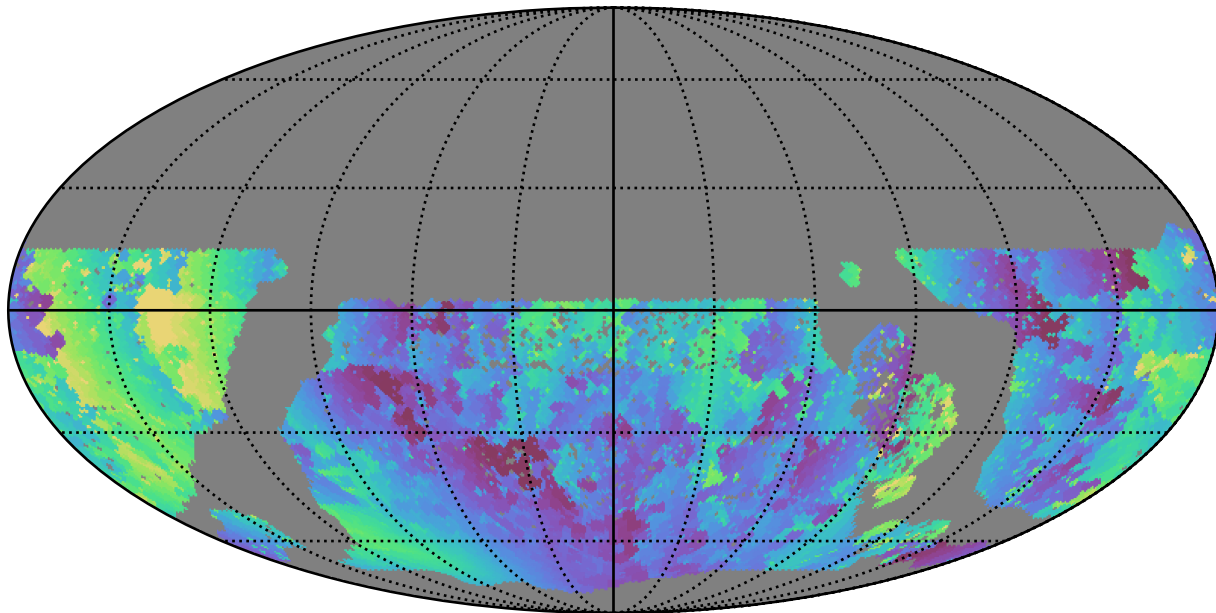
baseline_v3.2_10yrs WFD u band: Min solarElong
