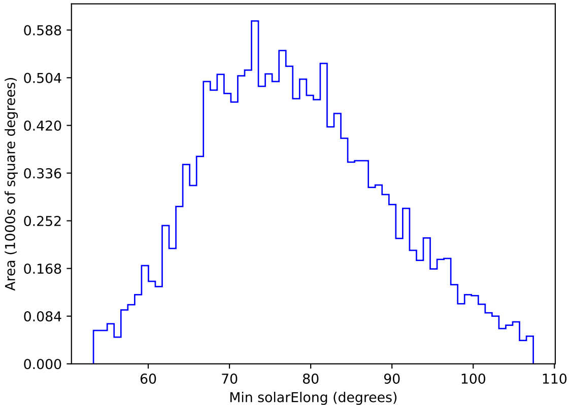
baseline_v3.2_10yrs WFD u band: Min solarElong
