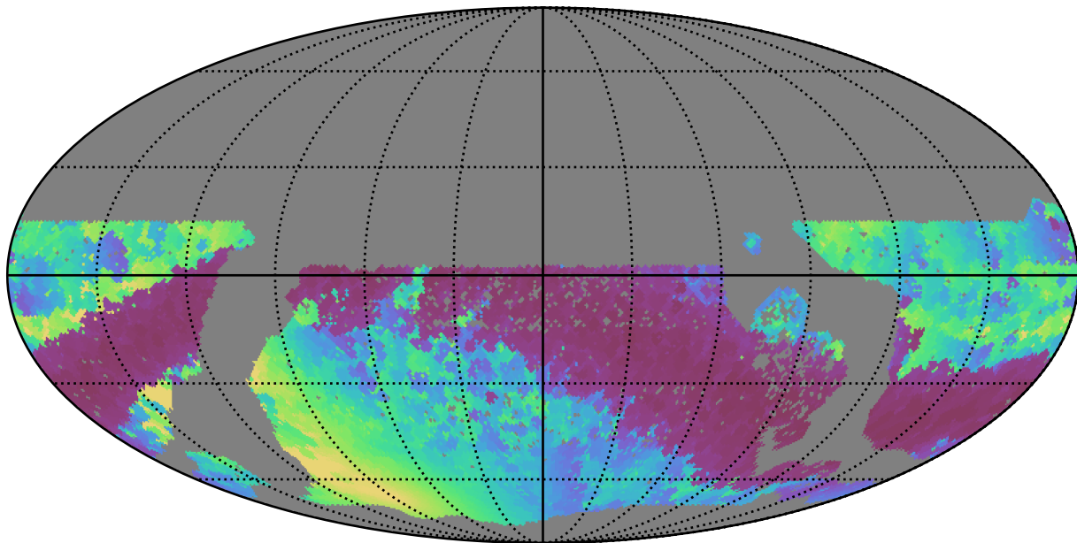
baseline_v3.2_10yrs WFD r band: Min solarElong
