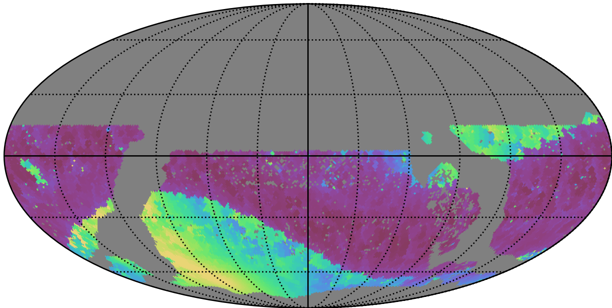
baseline_v3.2_10yrs WFD i band: Min solarElong
