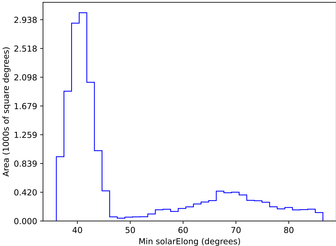
baseline_v3.2_10yrs WFD i band: Min solarElong
