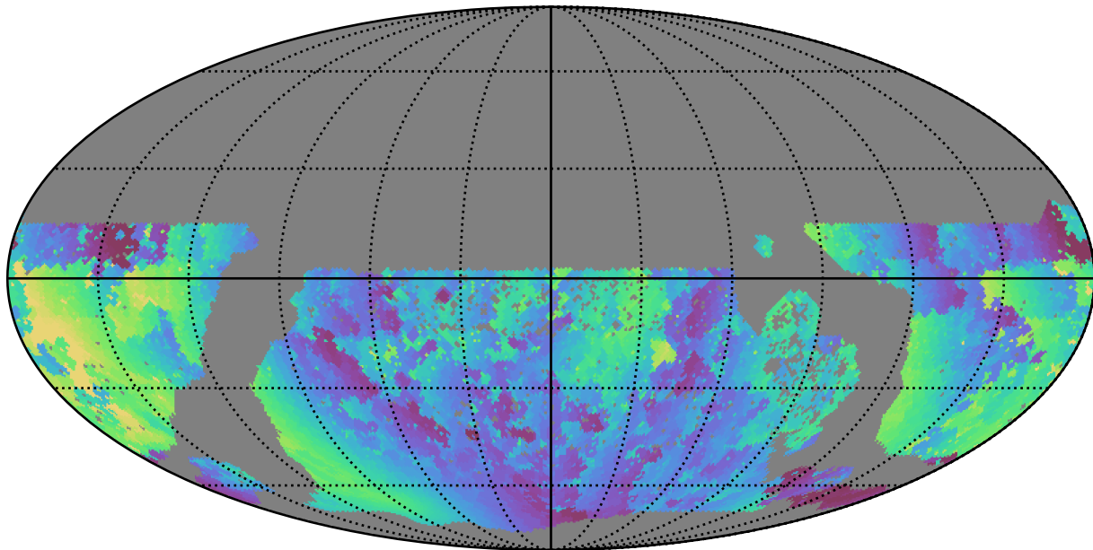
baseline_v3.2_10yrs WFD g band: Min solarElong
