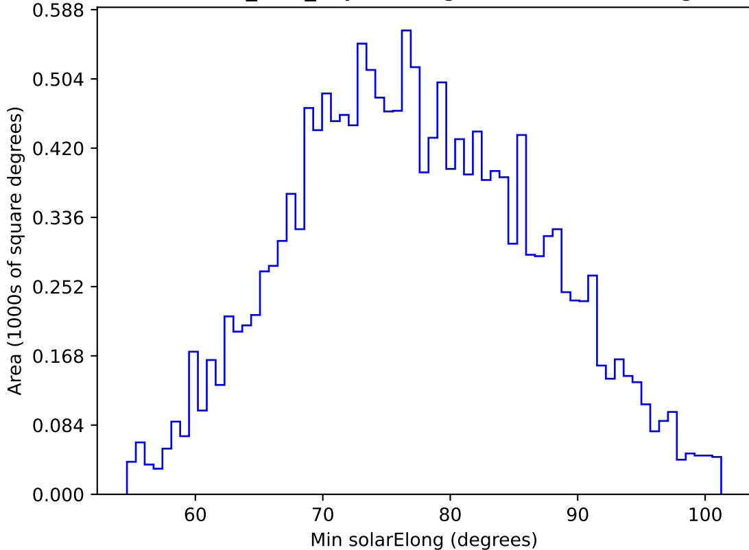
baseline_v3.2_10yrs WFD g band: Min solarElong
