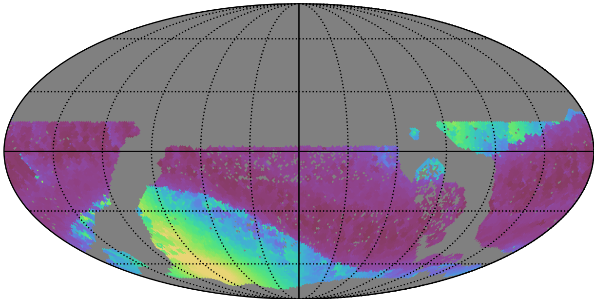
baseline_v3.2_10yrs WFD all bands: Min solarElong
