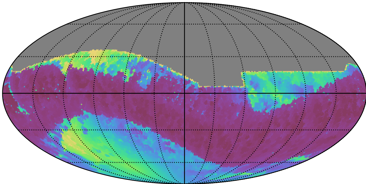
baseline_v3.2_10yrs All sky z band: Min solarElong
