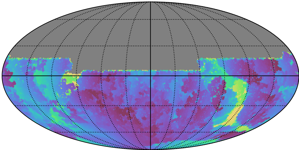
baseline_v3.2_10yrs All sky u band: Min solarElong
