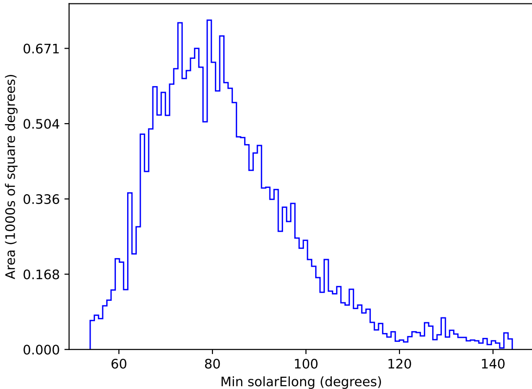
baseline_v3.2_10yrs All sky u band: Min solarElong
