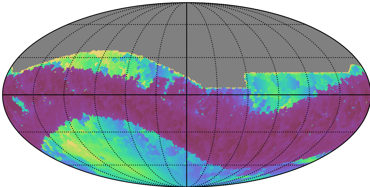
baseline_v3.2_10yrs All sky i band: Min solarElong
