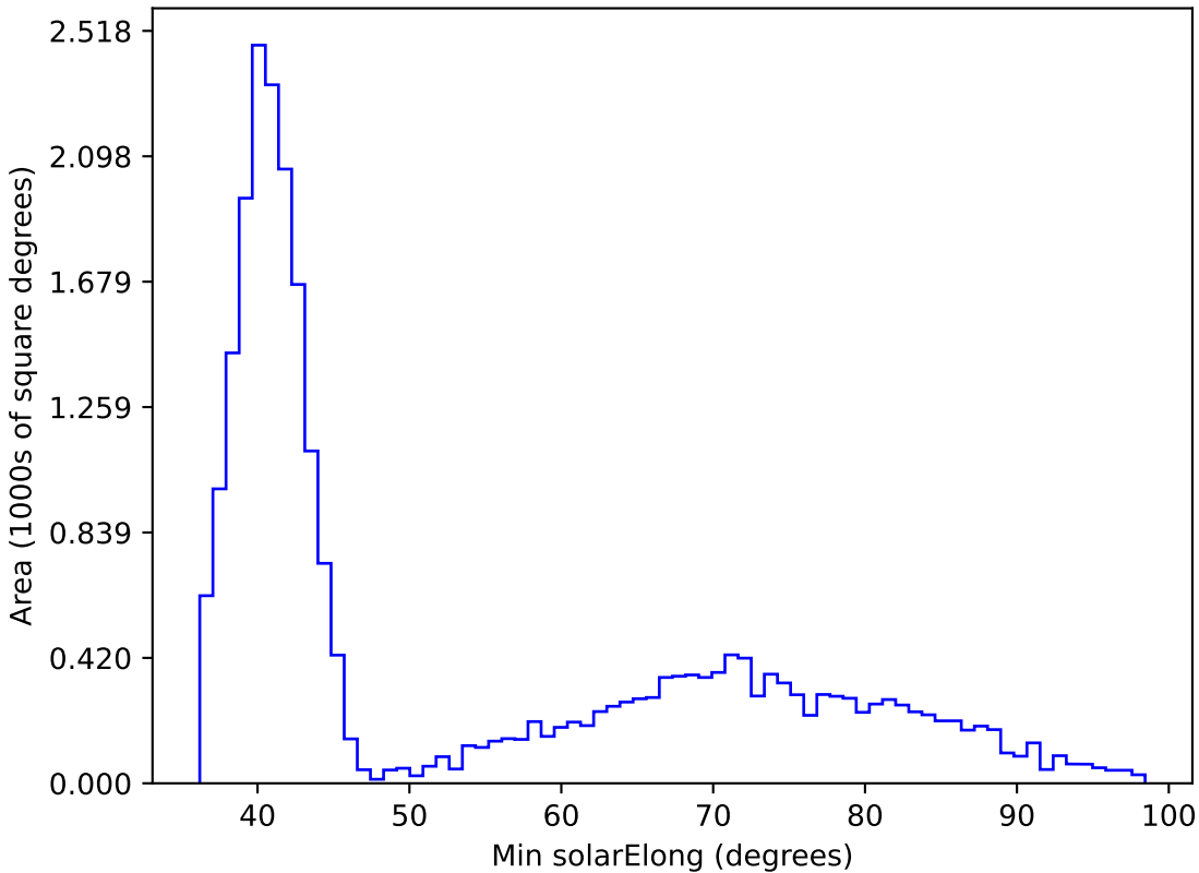
baseline_v3.2_10yrs All sky i band: Min solarElong
