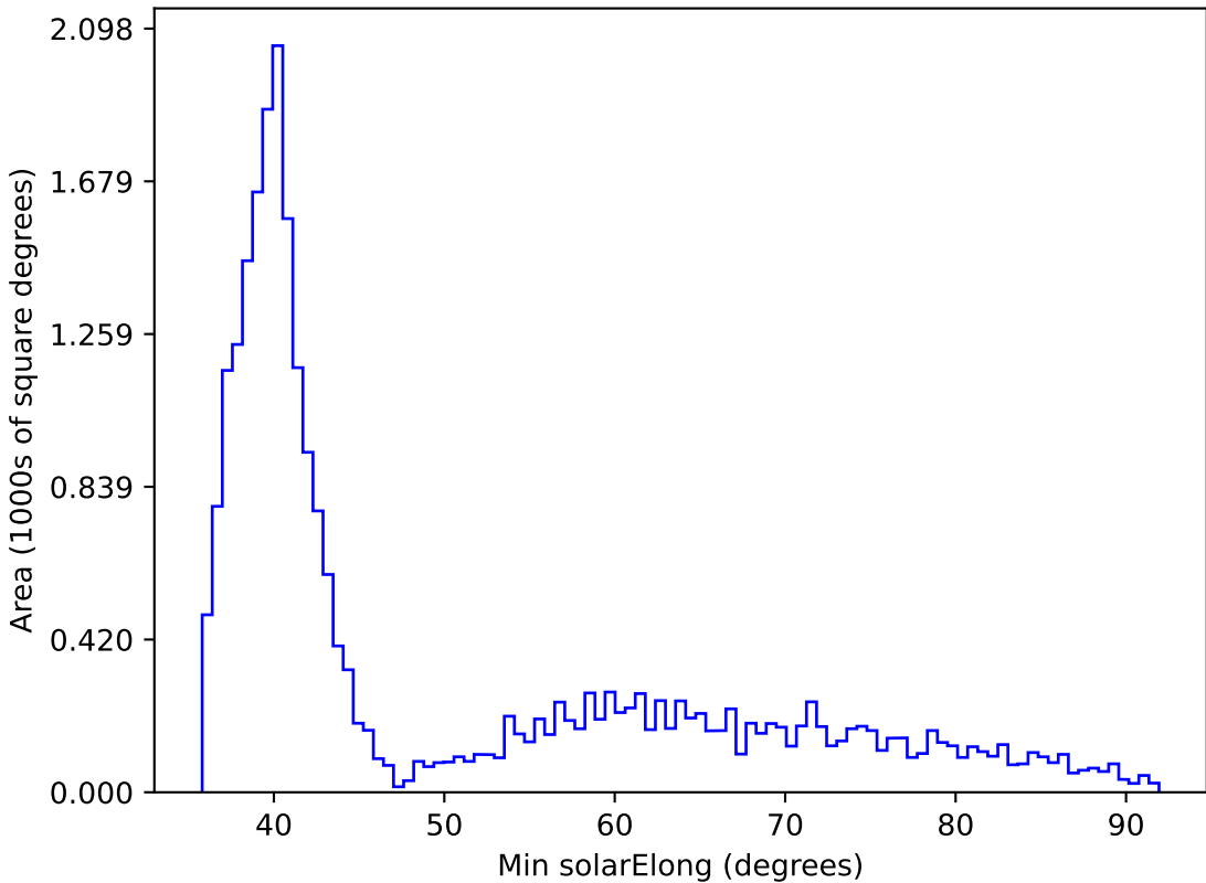
baseline_v3.2_10yrs All sky all bands: Min solarElong
