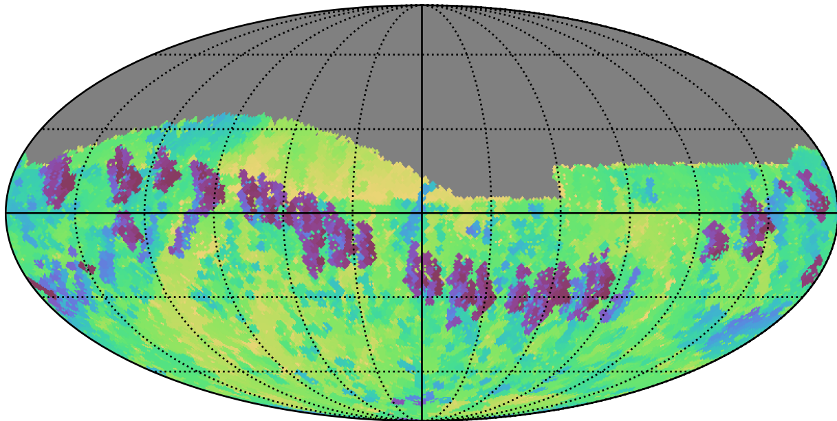
baseline_v3.2_10yrs Yr 1 z band: Min skyBrightness
