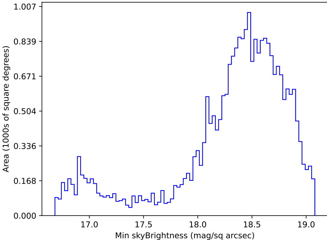
baseline_v3.2_10yrs Yr 1 z band: Min skyBrightness
