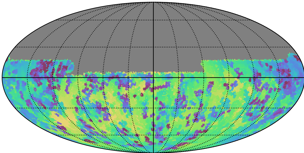
baseline_v3.2_10yrs Yr 1 y band: Min skyBrightness
