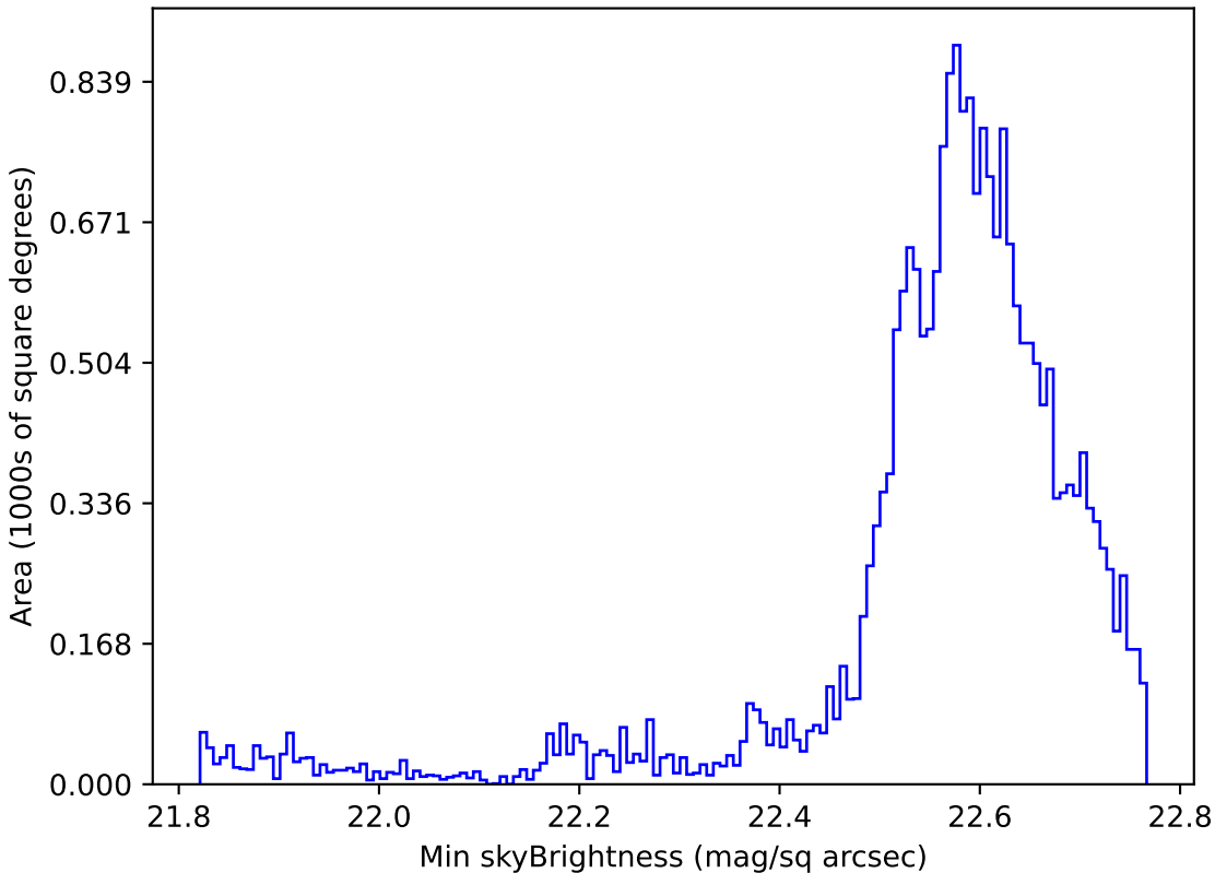
baseline_v3.2_10yrs Yr 1 u band: Min skyBrightness
