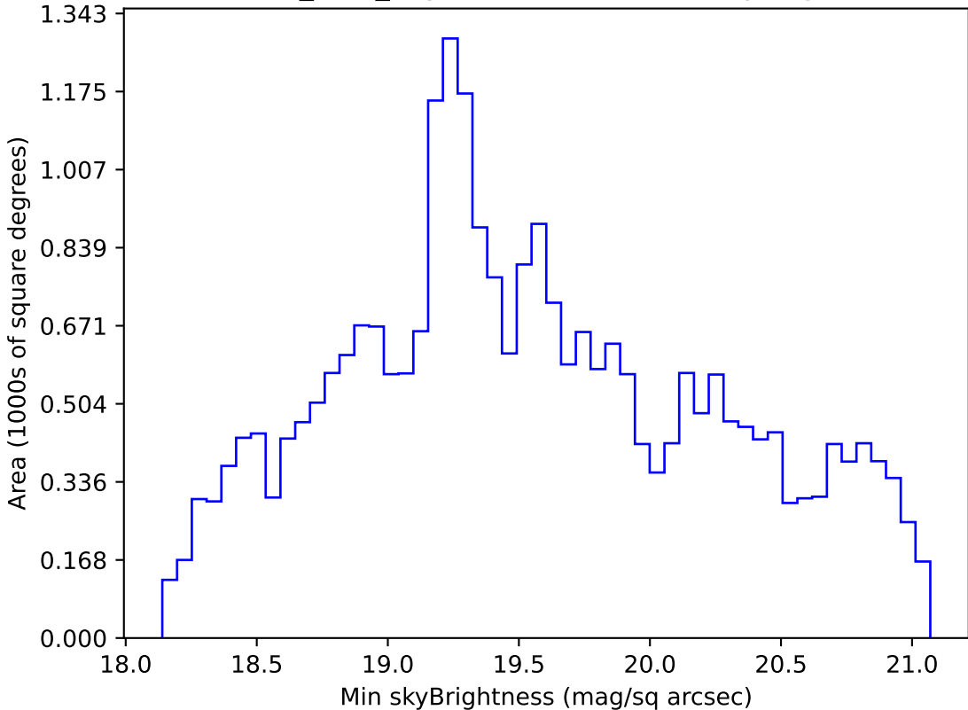
baseline_v3.2_10yrs Yr 1 r band: Min skyBrightness
