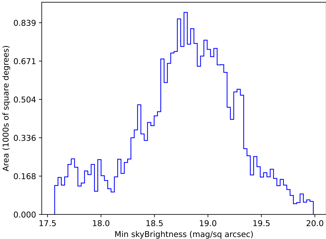
baseline_v3.2_10yrs Yr 1 i band: Min skyBrightness
