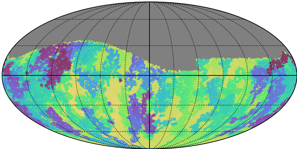
baseline_v3.2_10yrs Yr 1 g band: Min skyBrightness
