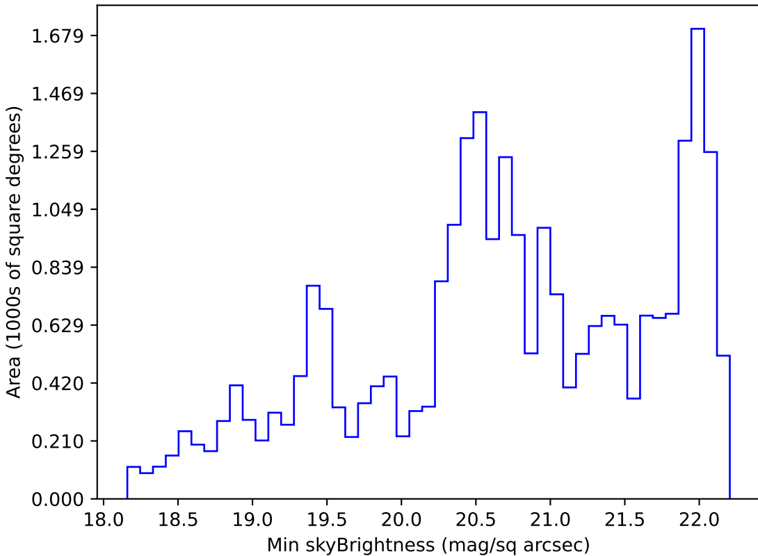
baseline_v3.2_10yrs Yr 1 g band: Min skyBrightness
