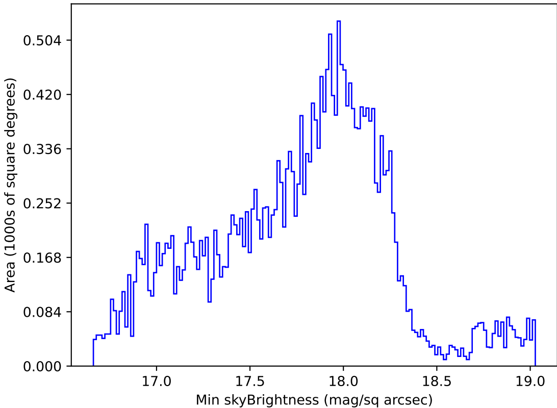
baseline_v3.2_10yrs Yr 1 all bands: Min skyBrightness
