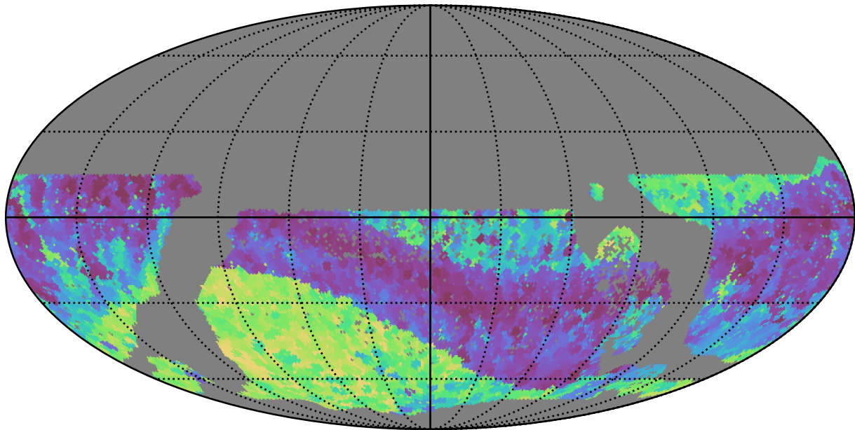
baseline_v3.2_10yrs WFD z band: Min skyBrightness
