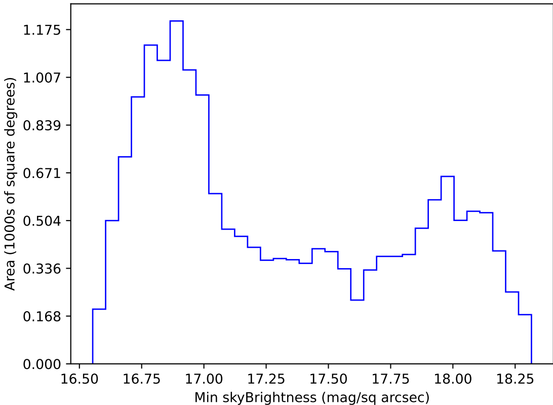
baseline_v3.2_10yrs WFD z band: Min skyBrightness
