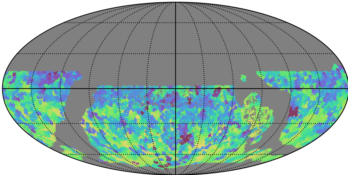
baseline_v3.2_10yrs WFD y band: Min skyBrightness
