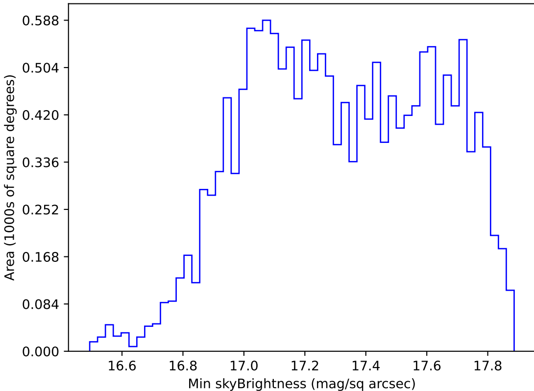
baseline_v3.2_10yrs WFD y band: Min skyBrightness
