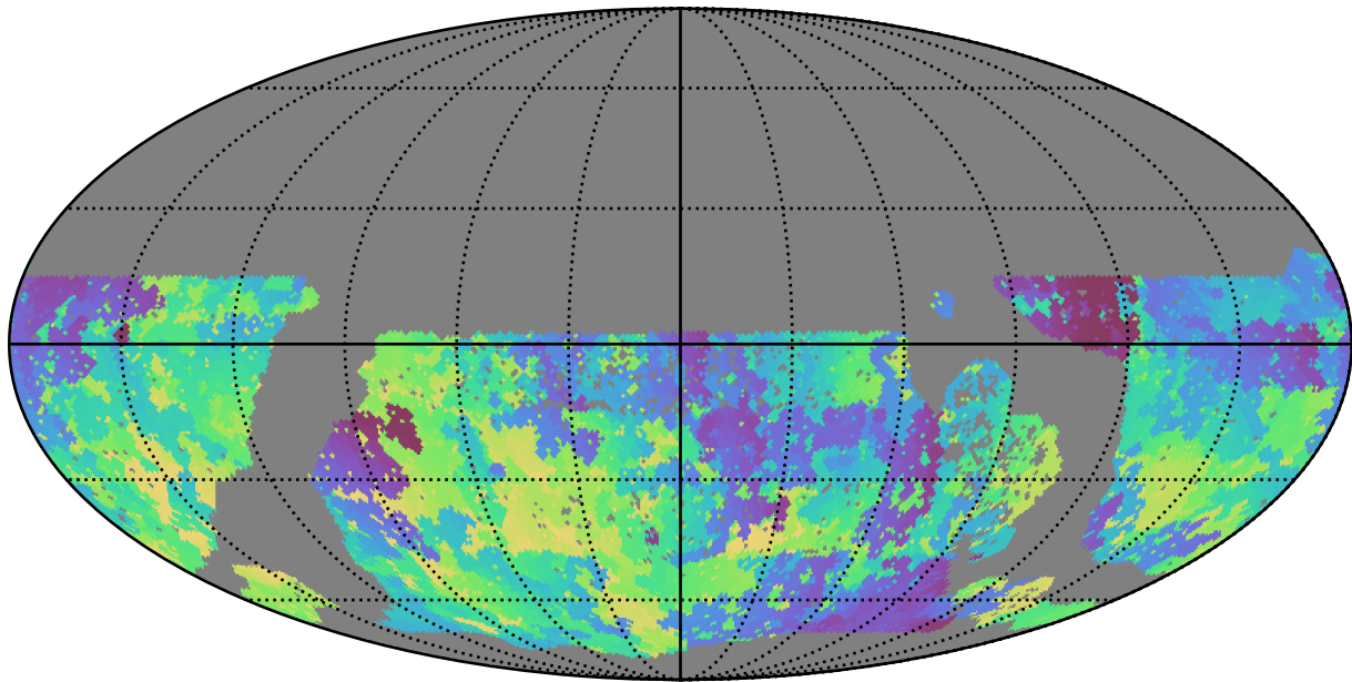
baseline_v3.2_10yrs WFD u band: Min skyBrightness
