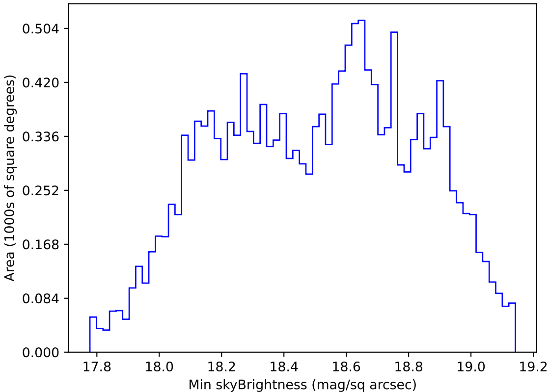
baseline_v3.2_10yrs WFD r band: Min skyBrightness
