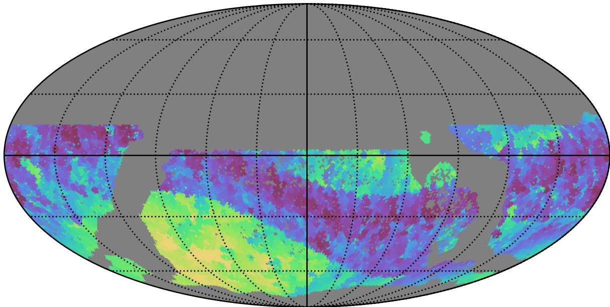
baseline_v3.2_10yrs WFD i band: Min skyBrightness
