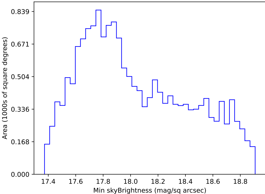
baseline_v3.2_10yrs WFD i band: Min skyBrightness
