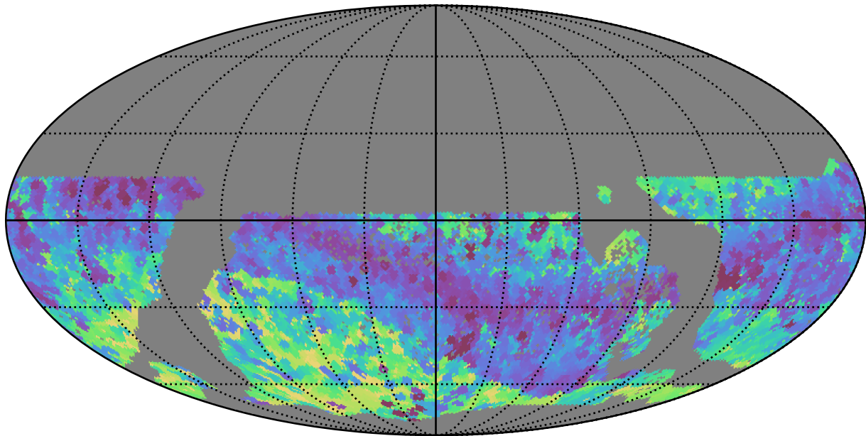
baseline_v3.2_10yrs WFD all bands: Min skyBrightness
