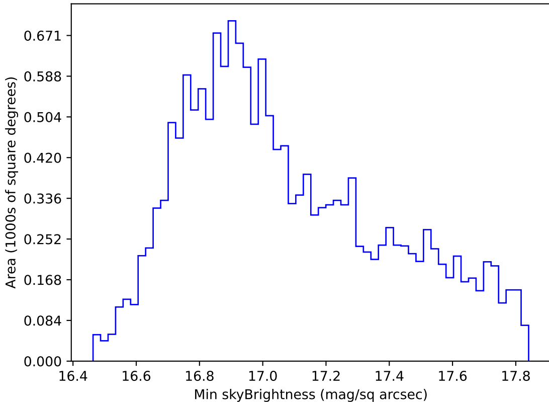
baseline_v3.2_10yrs WFD all bands: Min skyBrightness
