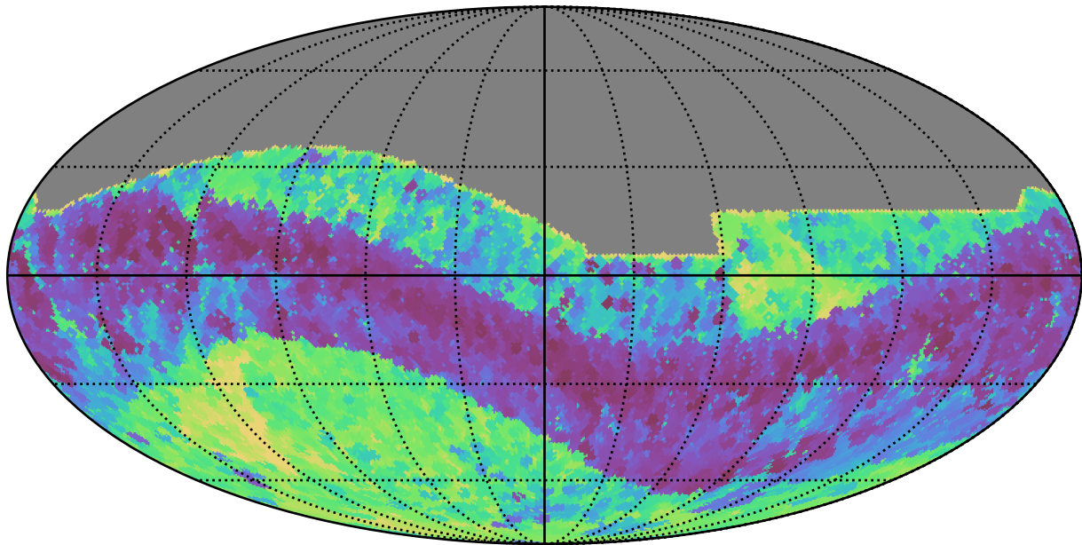
baseline_v3.2_10yrs All sky z band: Min skyBrightness
