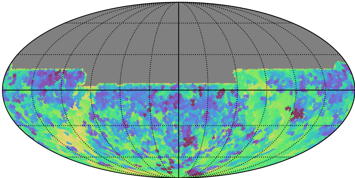
baseline_v3.2_10yrs All sky y band: Min skyBrightness
