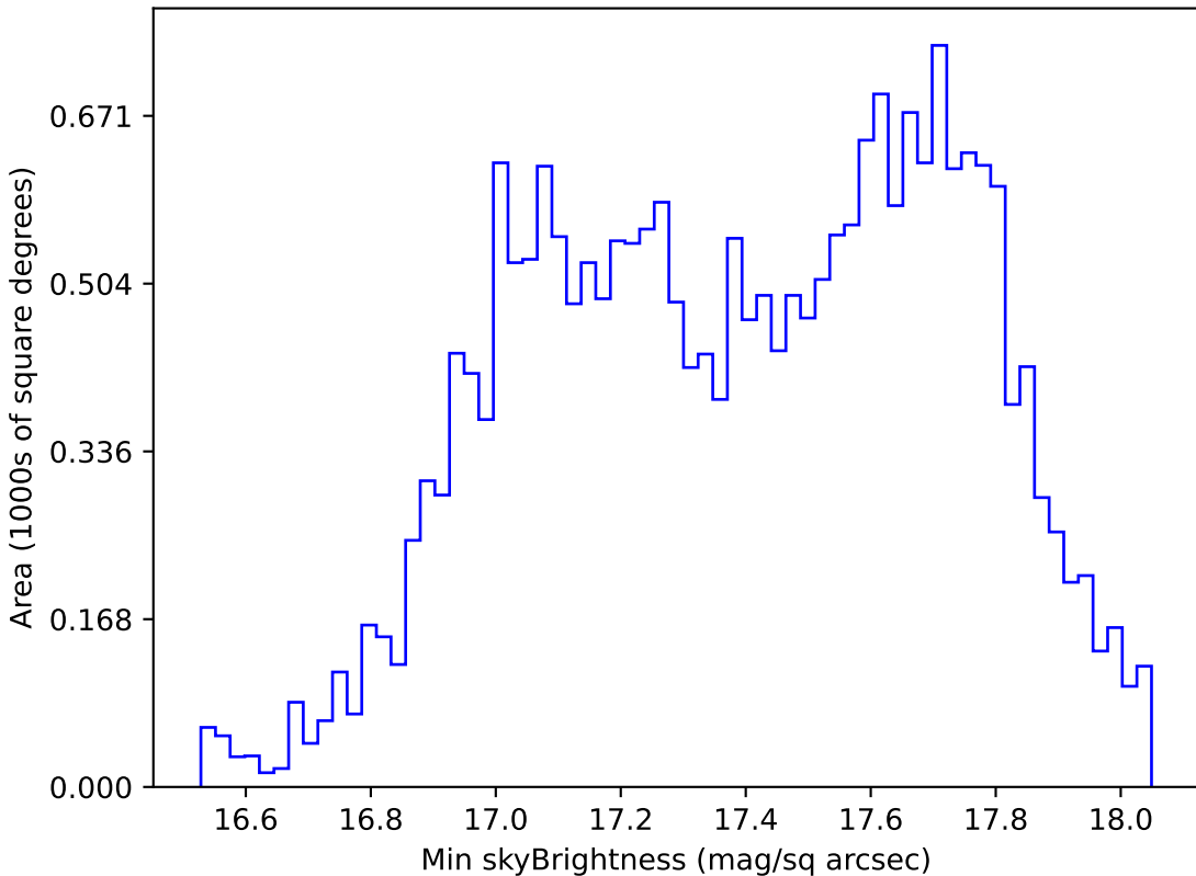
baseline_v3.2_10yrs All sky y band: Min skyBrightness
