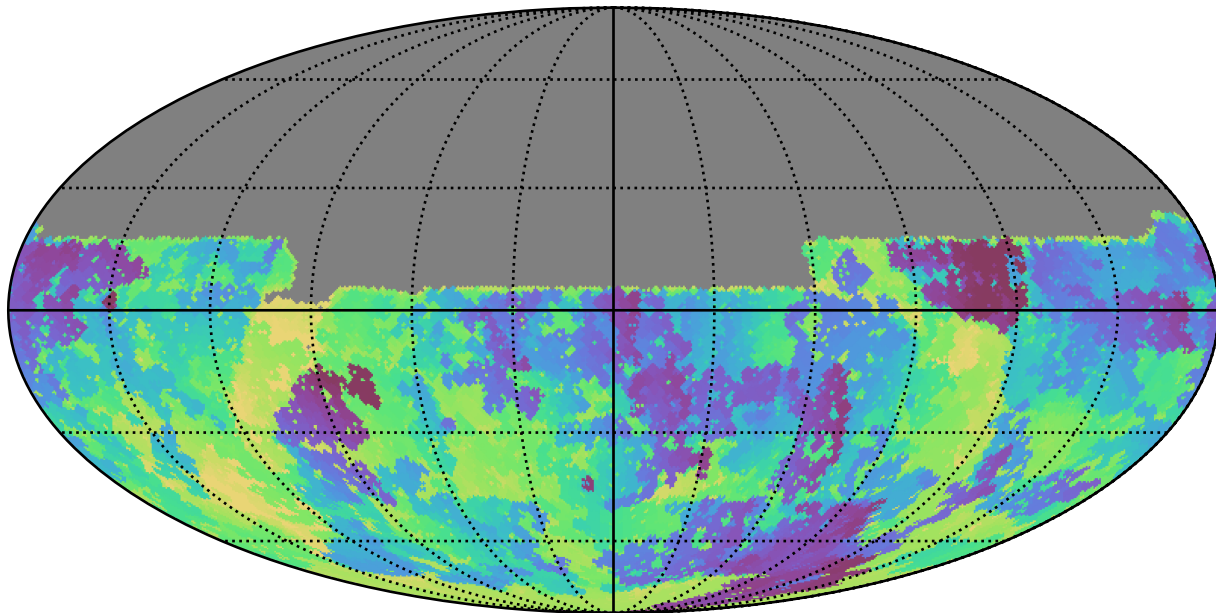
baseline_v3.2_10yrs All sky u band: Min skyBrightness
