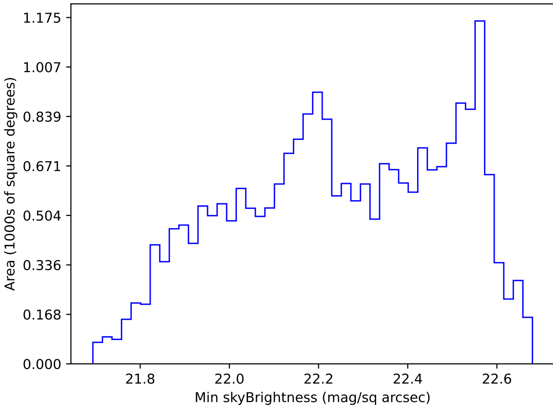
baseline_v3.2_10yrs All sky u band: Min skyBrightness
