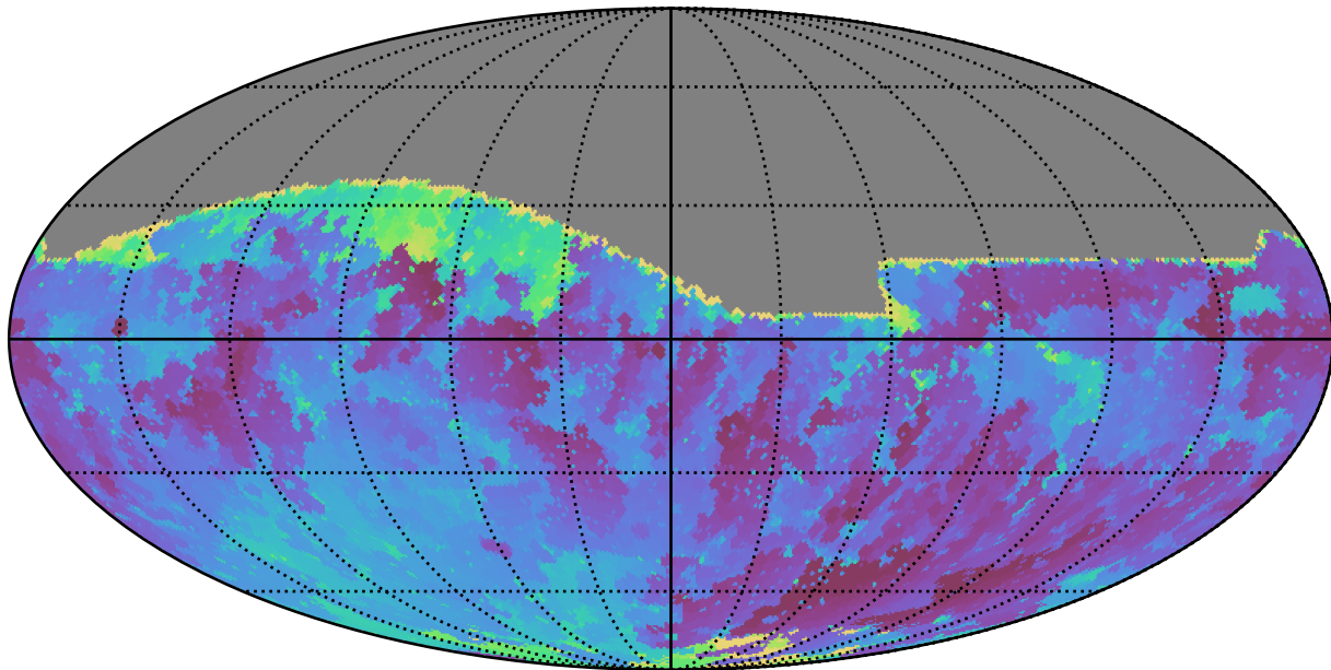
baseline_v3.2_10yrs All sky r band: Min skyBrightness
