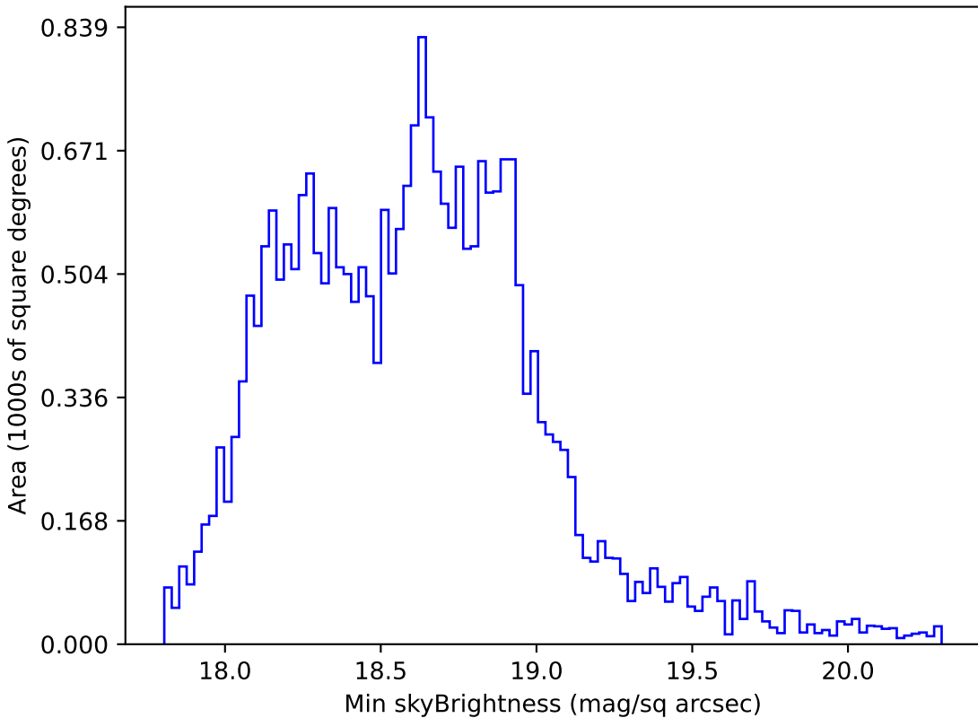
baseline_v3.2_10yrs All sky r band: Min skyBrightness
