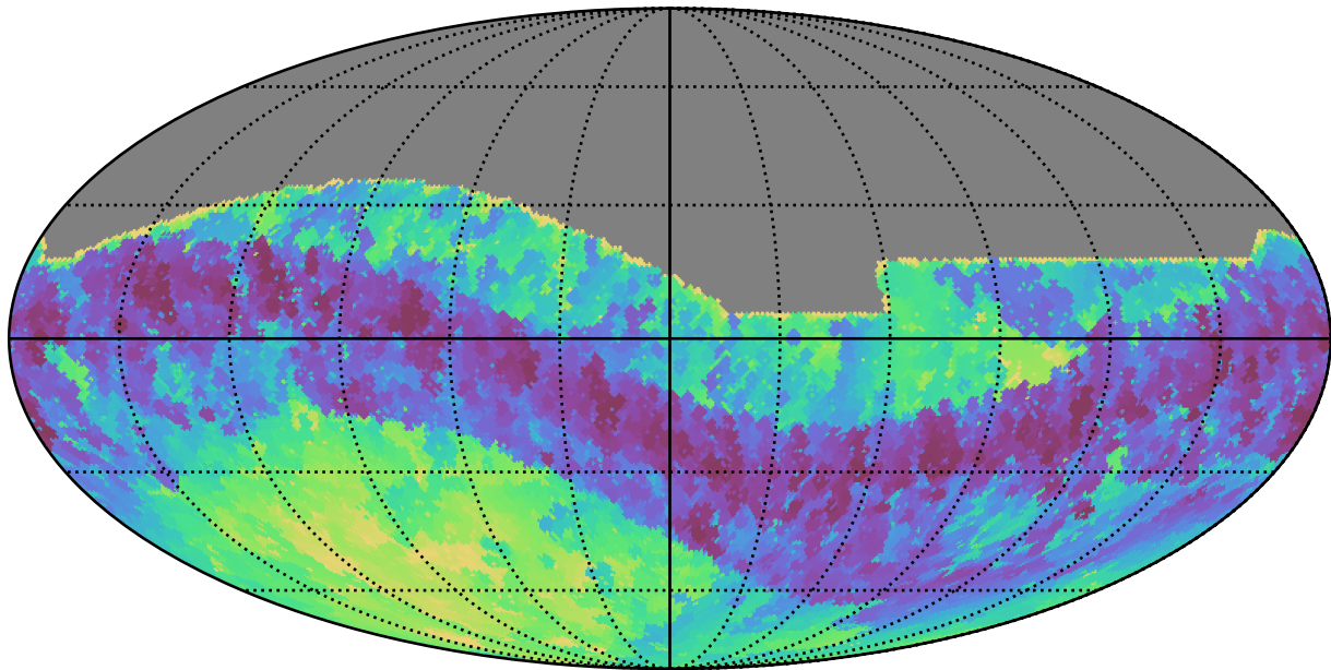
baseline_v3.2_10yrs All sky i band: Min skyBrightness
