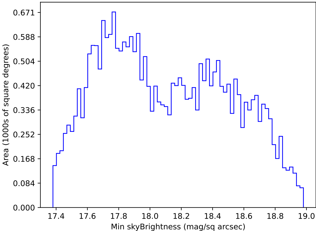
baseline_v3.2_10yrs All sky i band: Min skyBrightness
