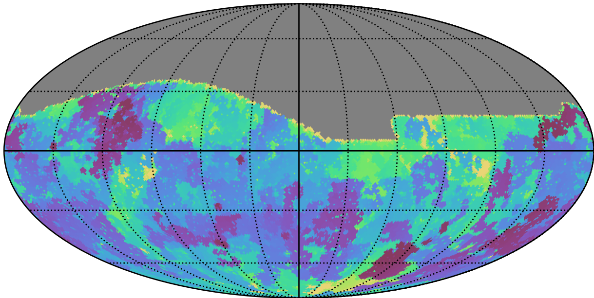
baseline_v3.2_10yrs All sky g band: Min skyBrightness
