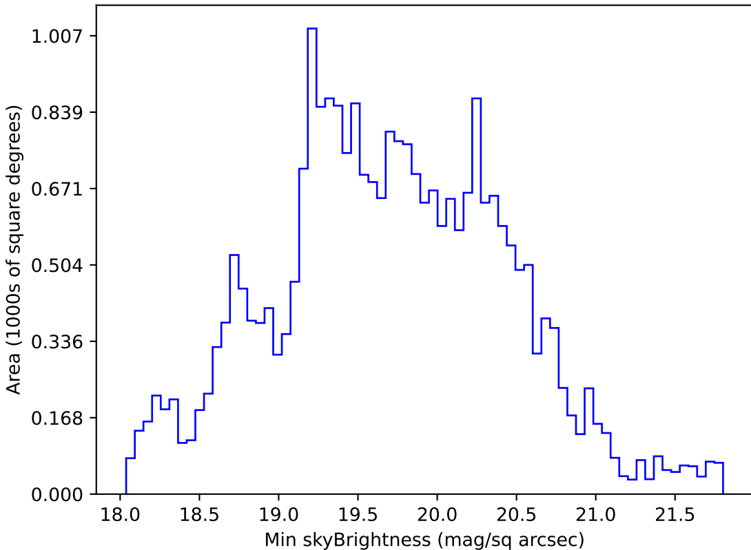
baseline_v3.2_10yrs All sky g band: Min skyBrightness
